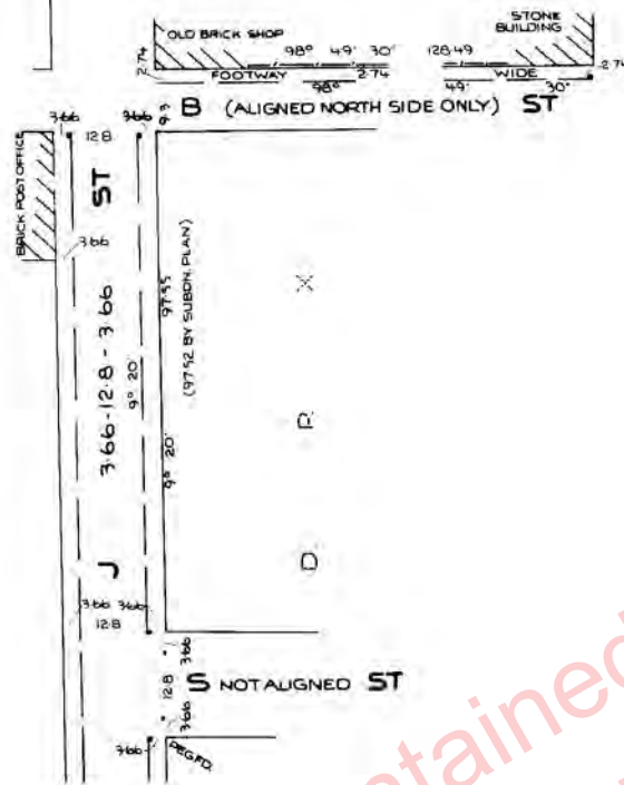
ALIGNMENT PLAN OF J ST AND NORTH SIDE OF B ST SURVEY 1912.
